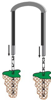
Hammer ground rods in, slide U-frame over top
